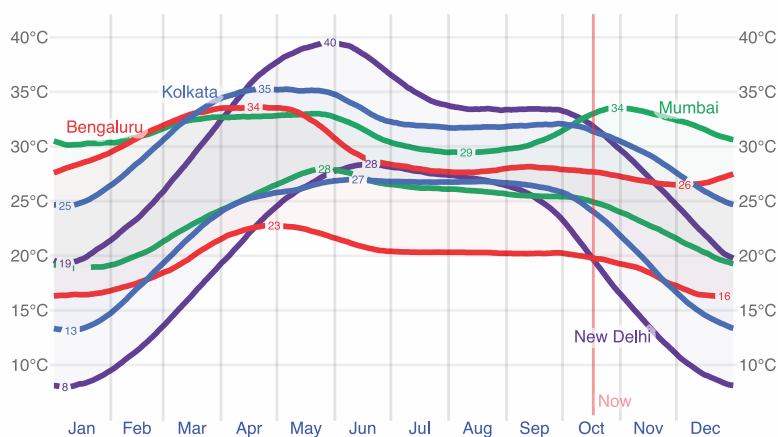
Average High and Low Temperature in India
