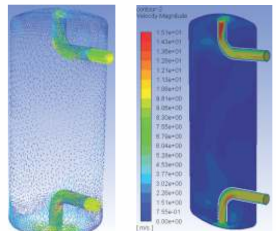
Velocity vector and Velocity contour of flow
